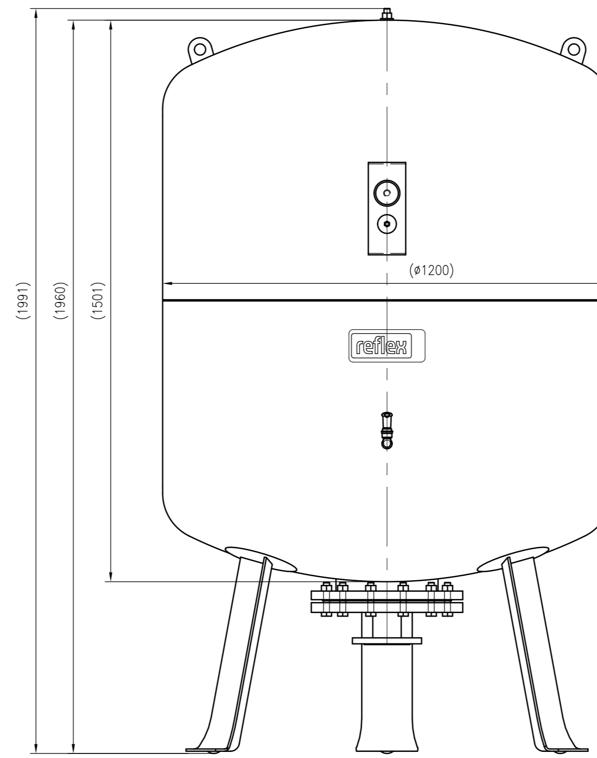
Front view
