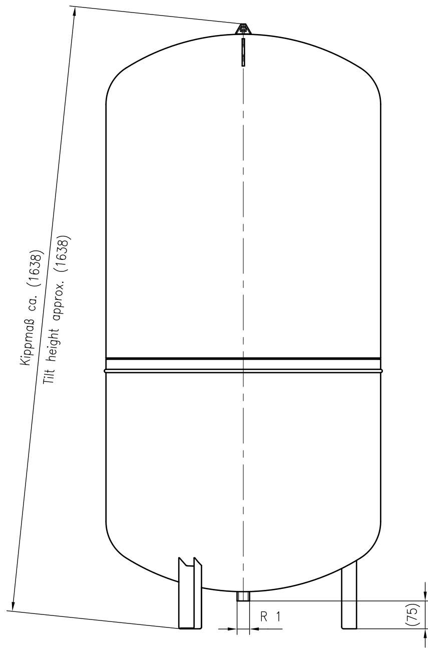
Side view
