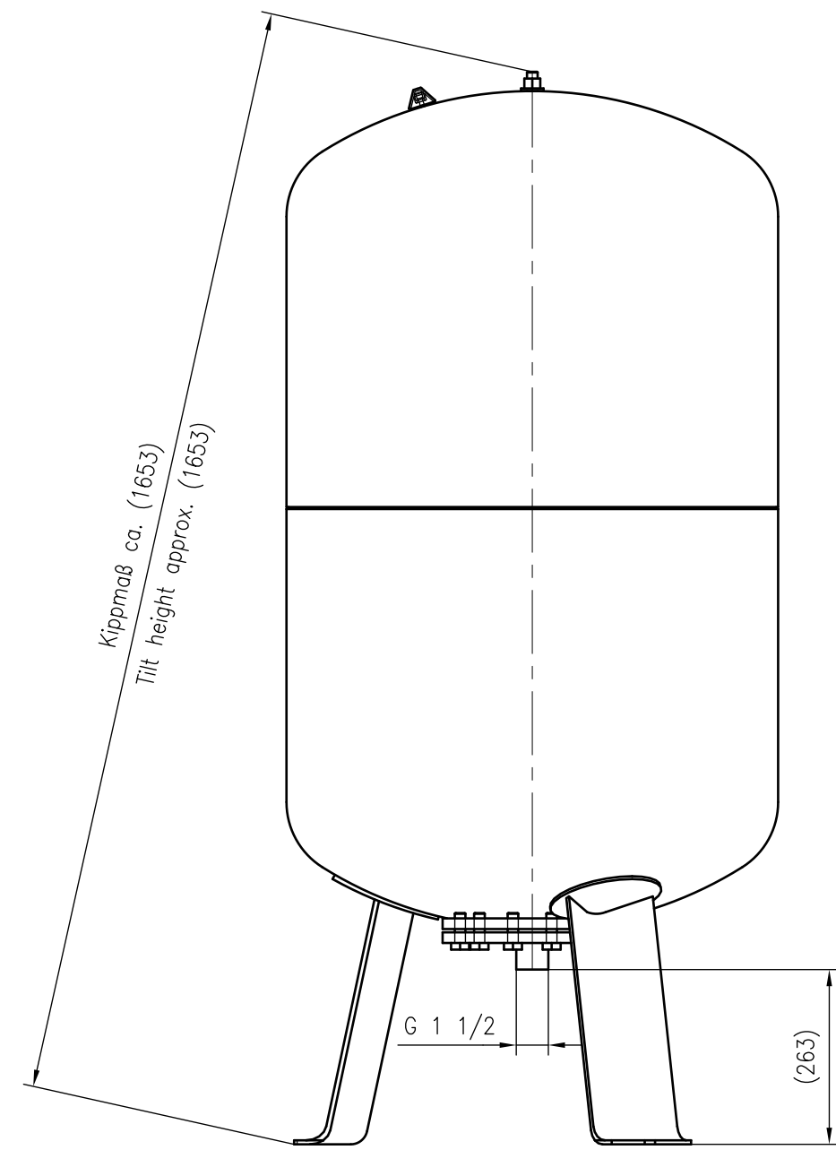
Side view
