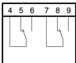
Auxillary contacts
